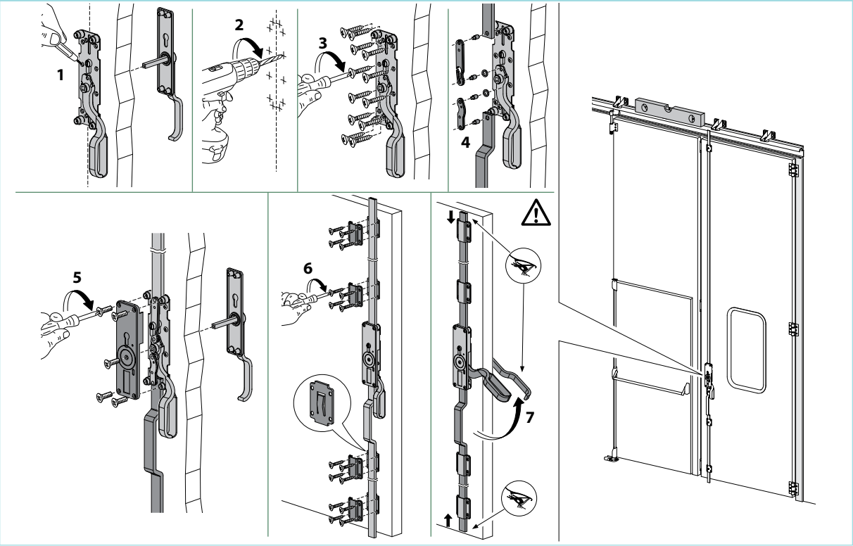
Mounting instructions art. 698 MC
